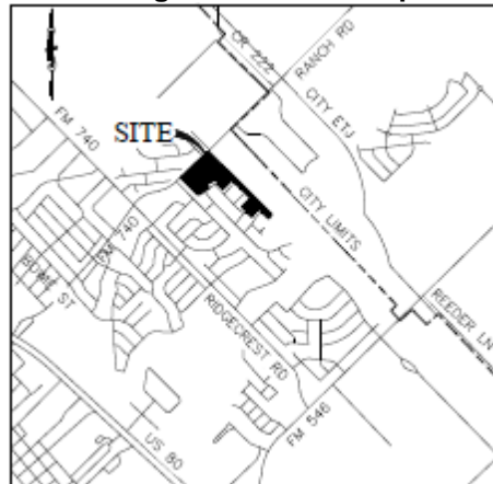
Image 1: Location Map
